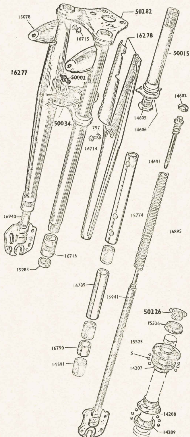
Front fork 50281
